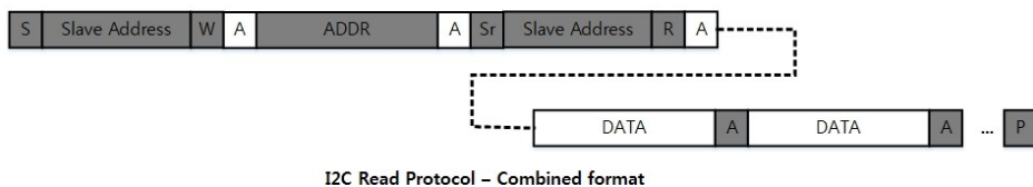
< Figure 4. I2C Protocols >
